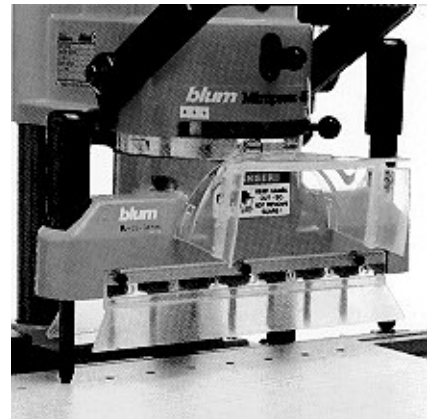
7 spindle line-boring head. TLB-MZK.1000
